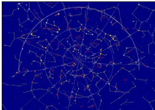
Figure 10. Celestial pole at midnight in January of 2798 BC, in Alpha Draconis.
